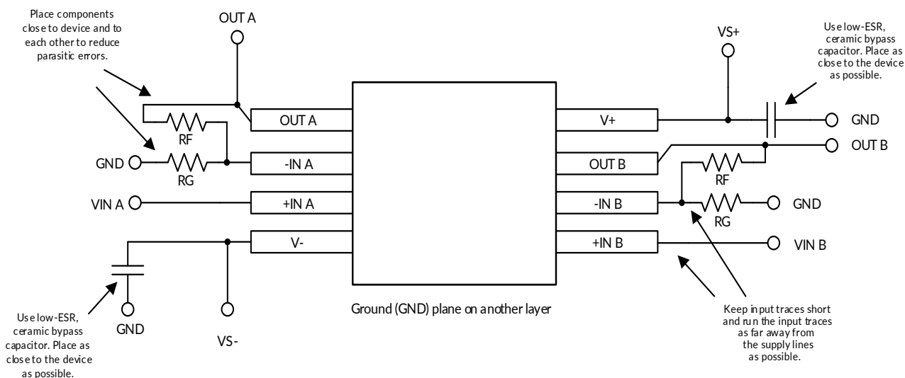
Figure 20. Layout Example
