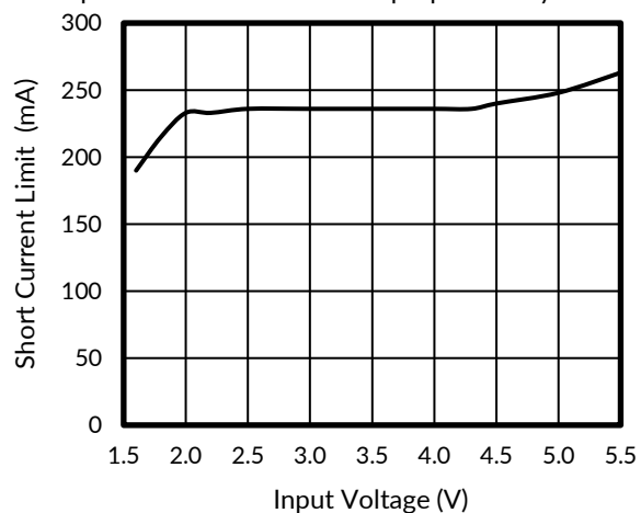
Figure 13. Short Current Limit vs Input Voltage
