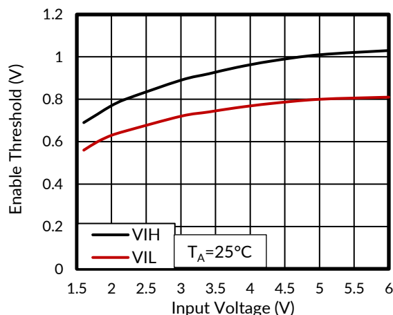
Figure 10. Enable Threshold vs Input Voltage
