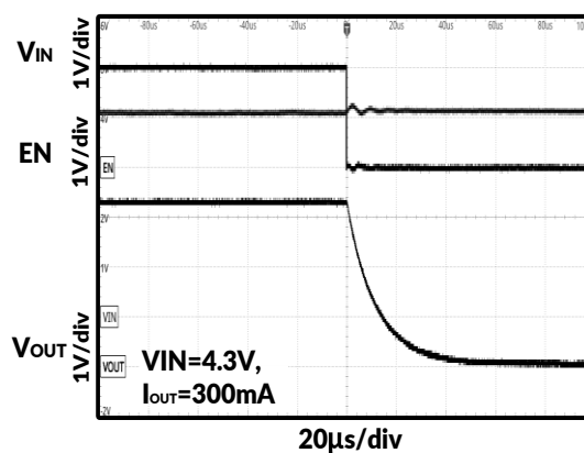
Figure 21. Turn Off
