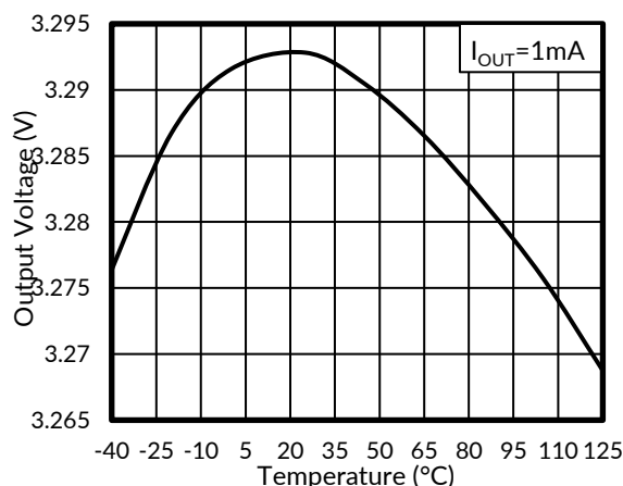
Figure 8. Output Voltage vs Junction Temperature
