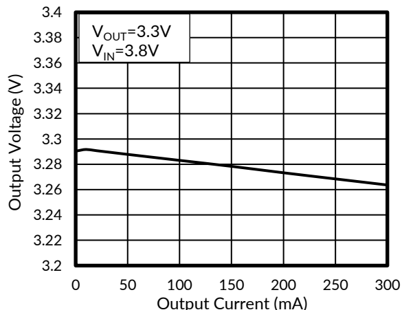
Figure 6. Load Regulation
