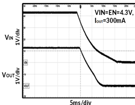
Figure 17. Power Off
