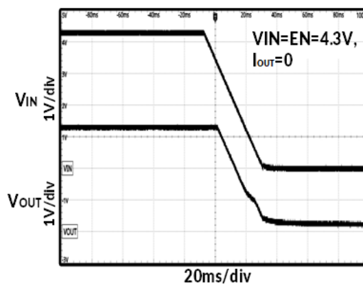
Figure 15. Power Off
