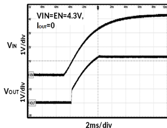
Figure 14. Power On
