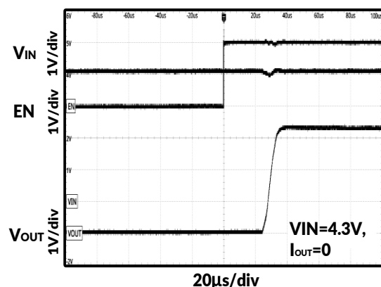
Figure 18. Turn On
