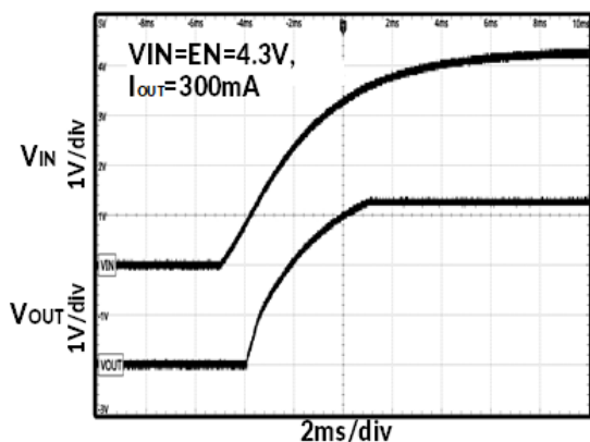
Figure 16. Power On
