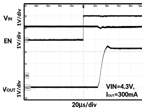
Figure 20. Turn On
