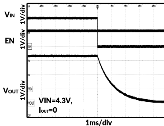
Figure 19. Turn Off
