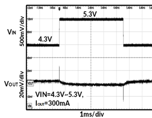
Figure 25. Line Transient Response ( I_{OUT}=300\text{mA} )
