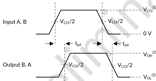
Figure 8. Propagation Delay
