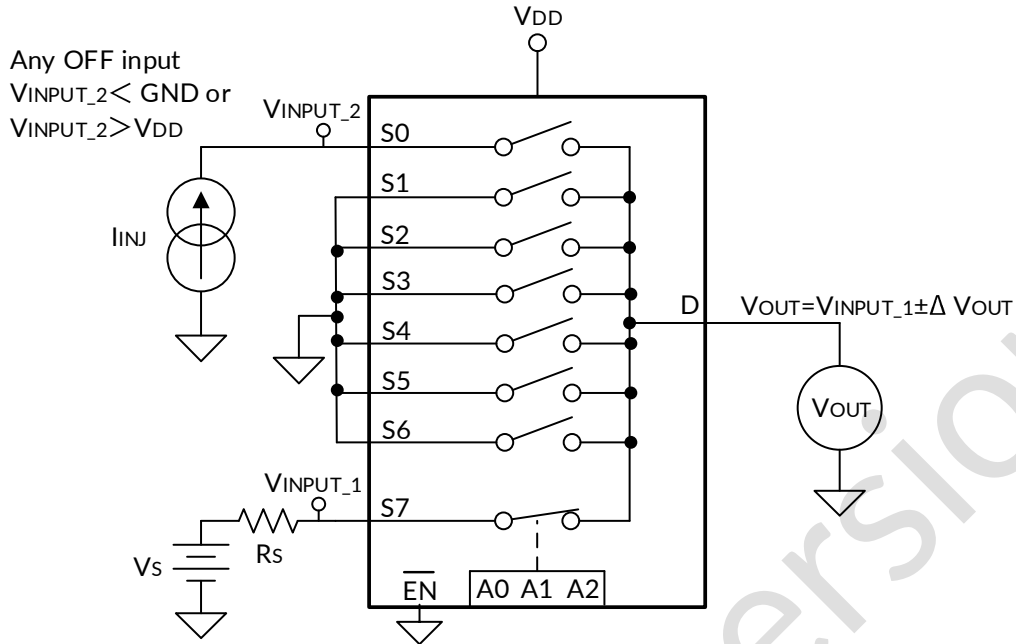
Figure 21. Injection Current Measurement Setup
