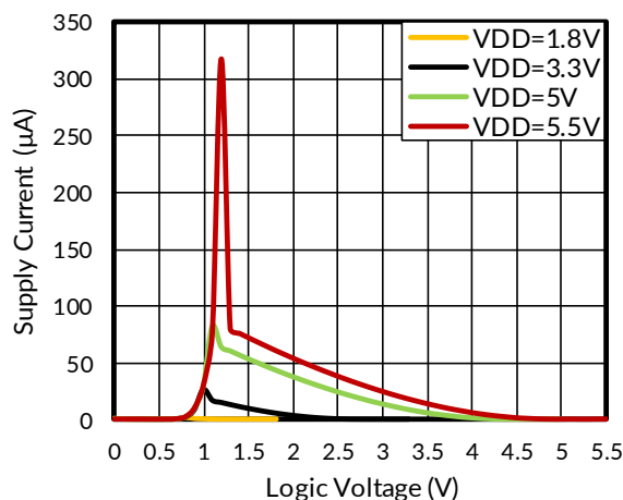
Figure 5. Supply Current vs Logic Voltage
