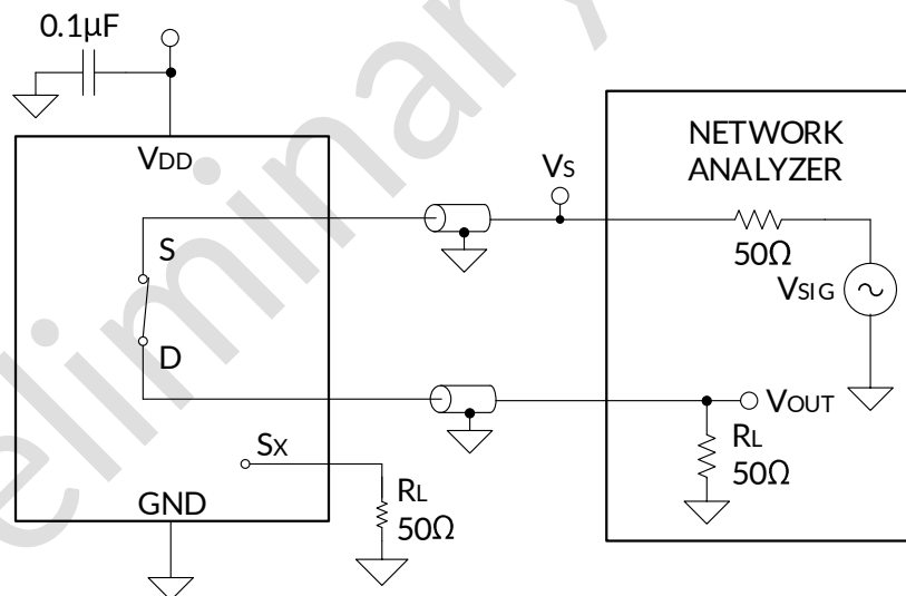
Figure 20. Bandwidth Measurement Setup
