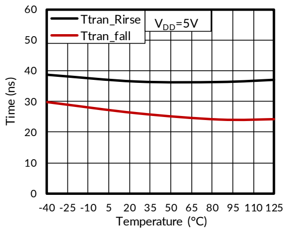
Figure 9. T_{TRANSITION} vs Temperature
