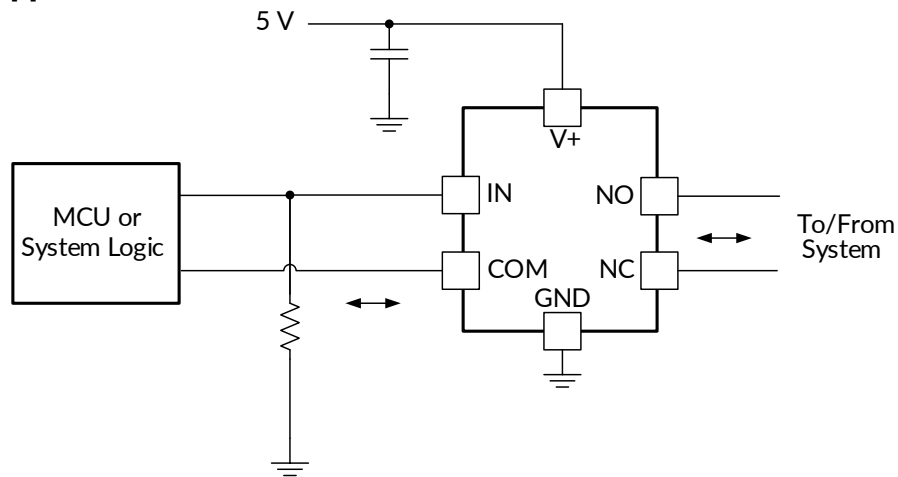
Figure 22. System Schematic for RS2057A
