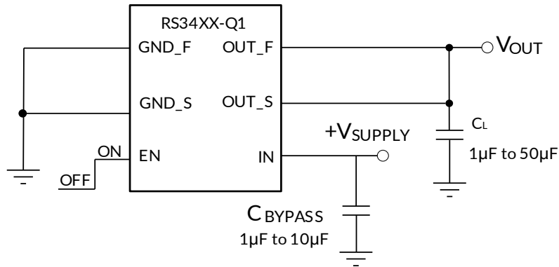
Figure 22. Basic Connections
