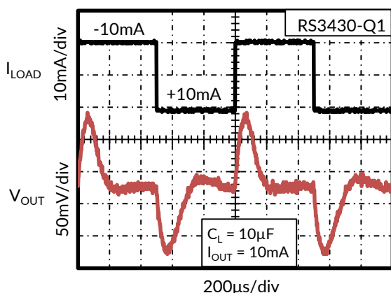
Figure 15. Load Transient
