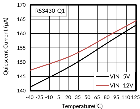
Figure 4. I_Q vs Temperature over V_{IN}
