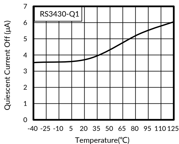
Figure 6. Quiescent Current Shutdown Mode
