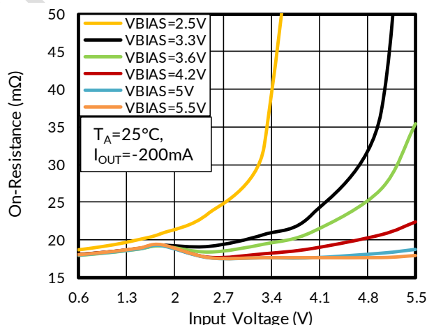
Figure 39. On-Resistance vs Input Voltage ( V_{IN} > V_{BIAS} Single Channel)
