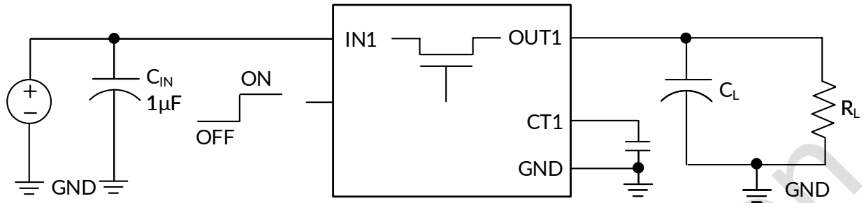
Figure 1. Test circuit
