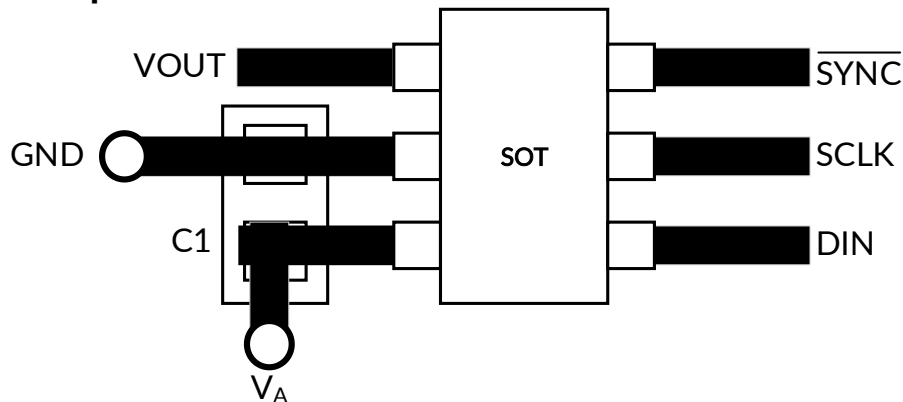
Figure 38. Typical Layout
