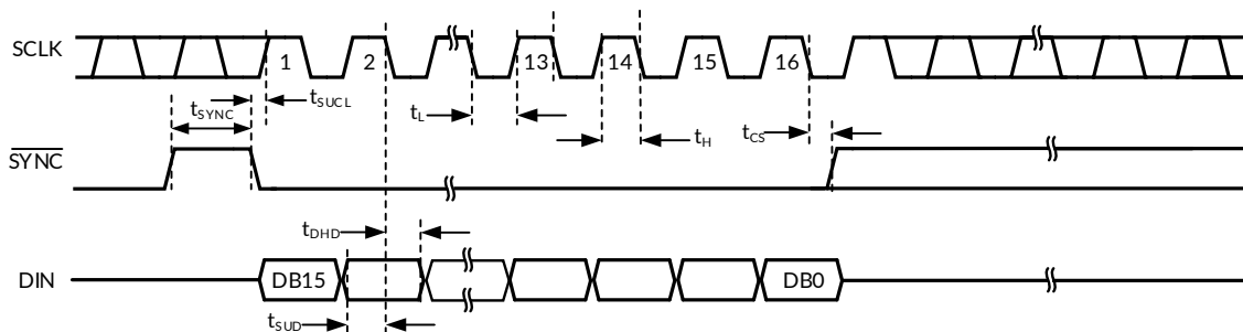
Figure 2. RS1320 Timing
