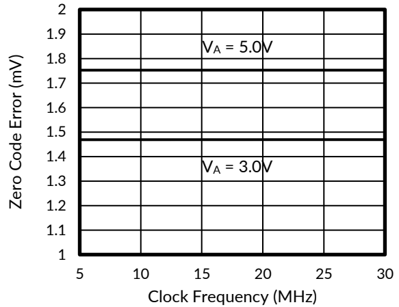
Figure 22. Zero Code Error vs f_{SCLK}
