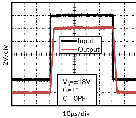
Figure 3. Large Signal Step Response
