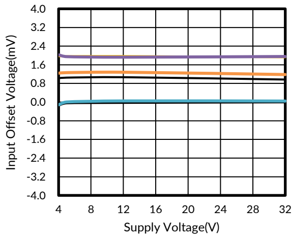
Figure 15. Input Offset Voltage vs Supply Voltage at 25^\circ\text{C}
