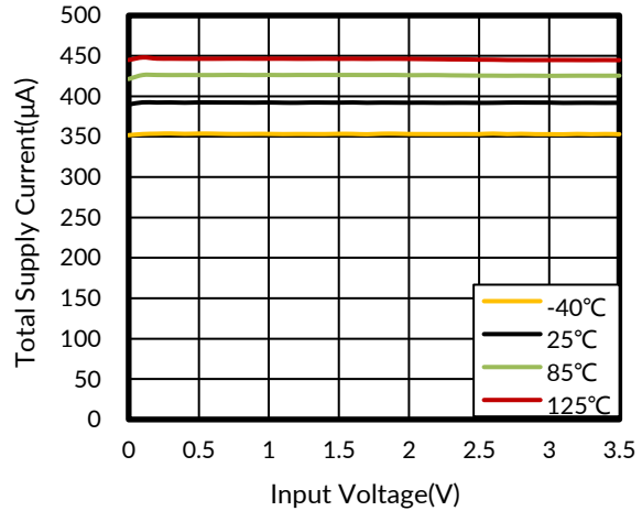
Figure 8. Total Supply Current vs Input Voltage at 5V
