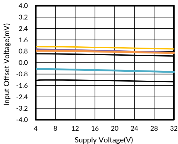
Figure 17. Input Offset Voltage vs Supply Voltage at 125^\circ\text{C}
