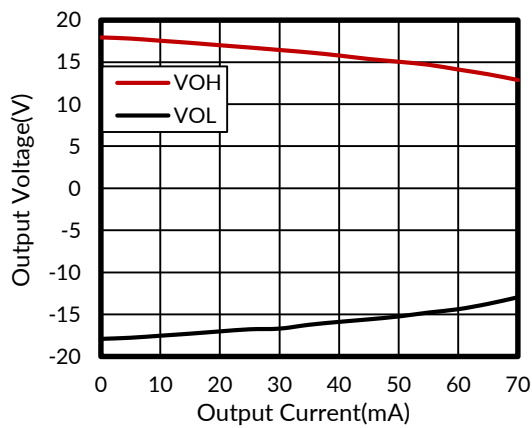
Figure 9. Output Voltage Swing vs Output Current
